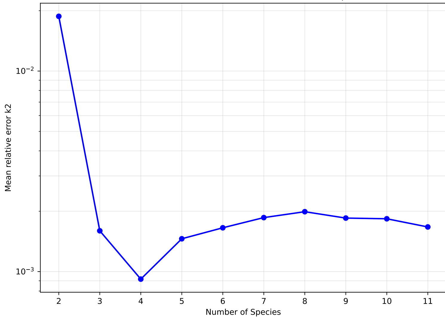
30, 30 — Mean relative error k2 vs number of species
